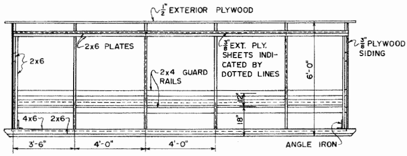
BACK SIDE FRAMING
