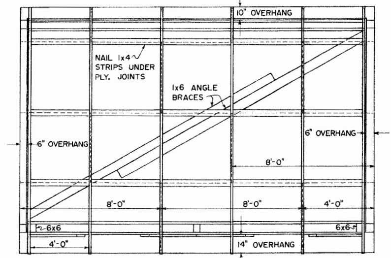
ROOF FRAMING
