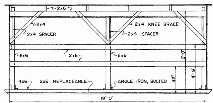
FRONT SIDE FRAMING
